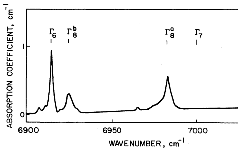
FIG. 1. Absorption spectrum of \text{Co}^{2+} in \text{KMgF}_3 in the region of the {}^4T_1(\Gamma_6) \rightarrow {}^4T_2 no-phonon lines. T = 1.8^\circ\text{K} , specimen thickness = 6.5 mm, and cobalt concentration is approximately 0.03 at. %.
