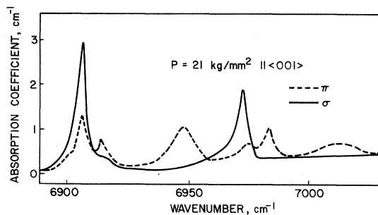
FIG. 2. Effect of applying a stress of 21\text{ kg/mm}^2 parallel to \langle 001 \rangle on the {}^4T_1(\Gamma_6) \rightarrow {}^4T_2 no-phonon lines of \text{Co}^{2+} in \text{KMgF}_3 . Full line: \sigma polarization ( \text{H} \parallel p ); dashed line: \pi polarization ( \text{H} \perp p ). \text{H} is the magnetic vector of the light. Note the extra \pi -polarized line at 7013\text{ cm}^{-1} . T = 1.8^\circ\text{K} , cobalt concentration is approximately 0.1 at. %.
